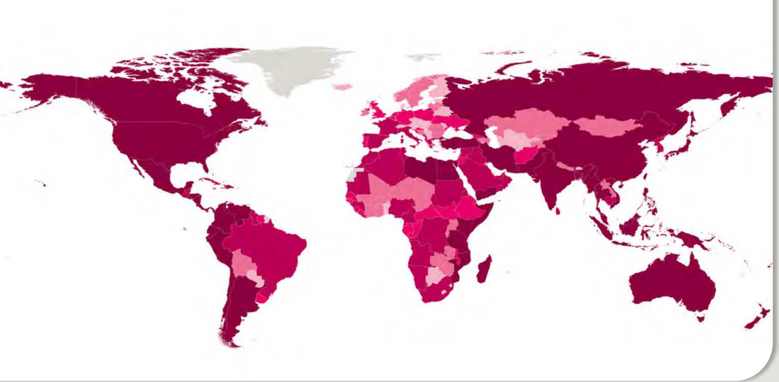
Figure 1: The WorldRiskIndex 2022
